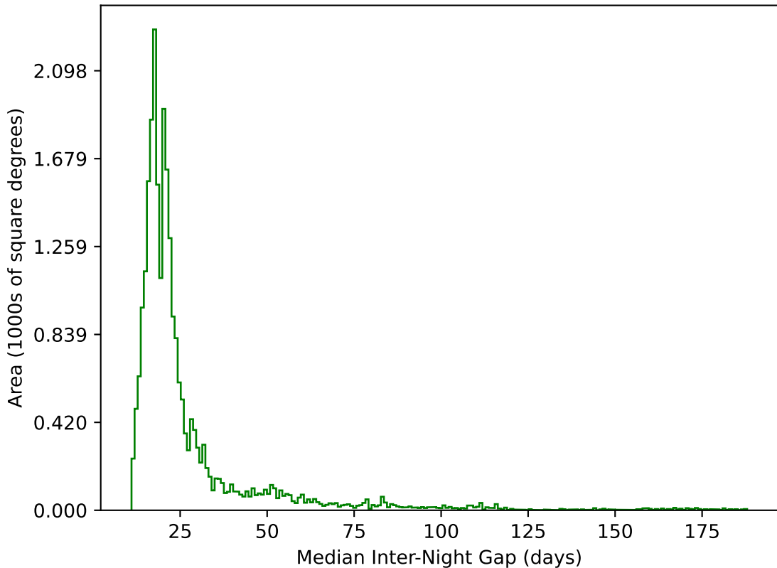
roll_pause_mjdp365_v3.4_10yrs All sky g band: Median Inter-Night Gap
