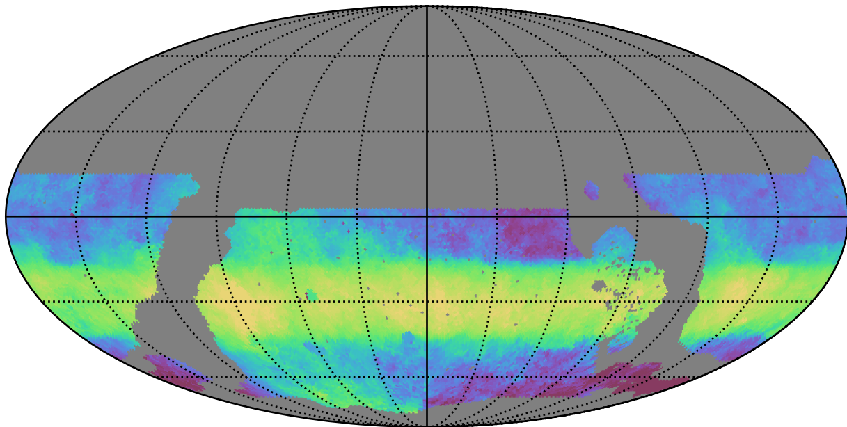
roll_pause_mjdp365_v3.4_10yrs WFD z band: Median HA
