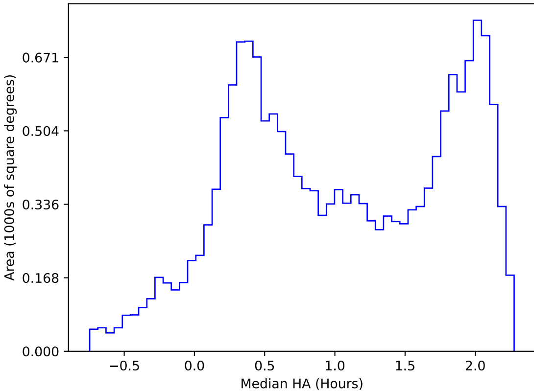
roll_pause_mjdp365_v3.4_10yrs WFD z band: Median HA
