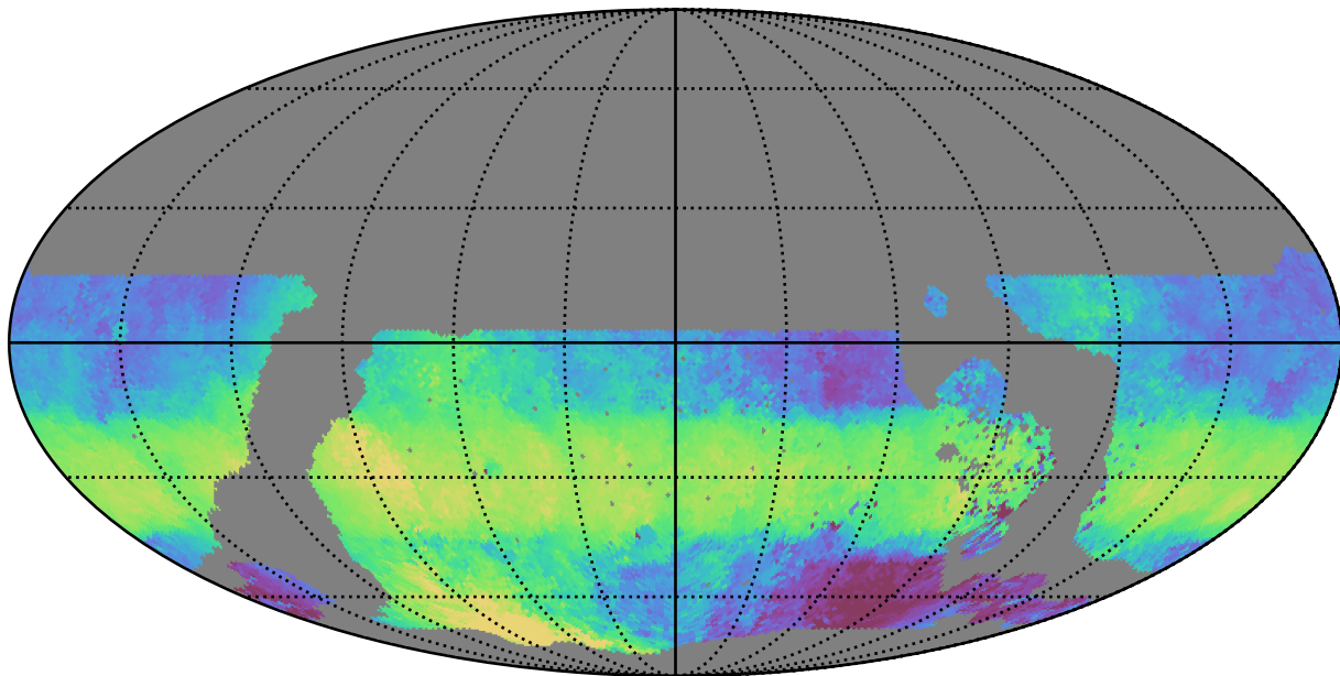
roll_pause_mjdp365_v3.4_10yrs WFD u band: Median HA
