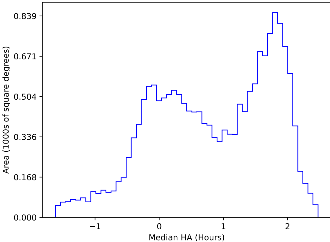
roll_pause_mjdp365_v3.4_10yrs WFD u band: Median HA
