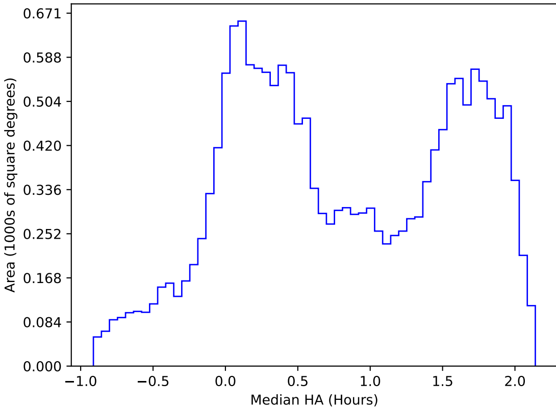
roll_pause_mjdp365_v3.4_10yrs WFD r band: Median HA
