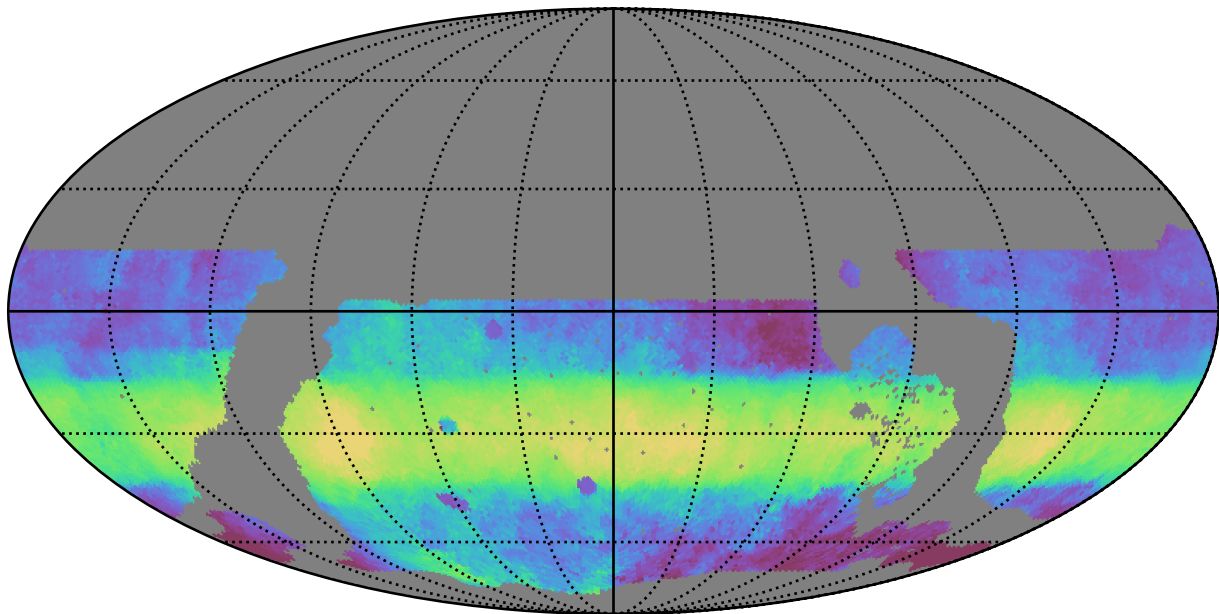
roll_pause_mjdp365_v3.4_10yrs WFD i band: Median HA
