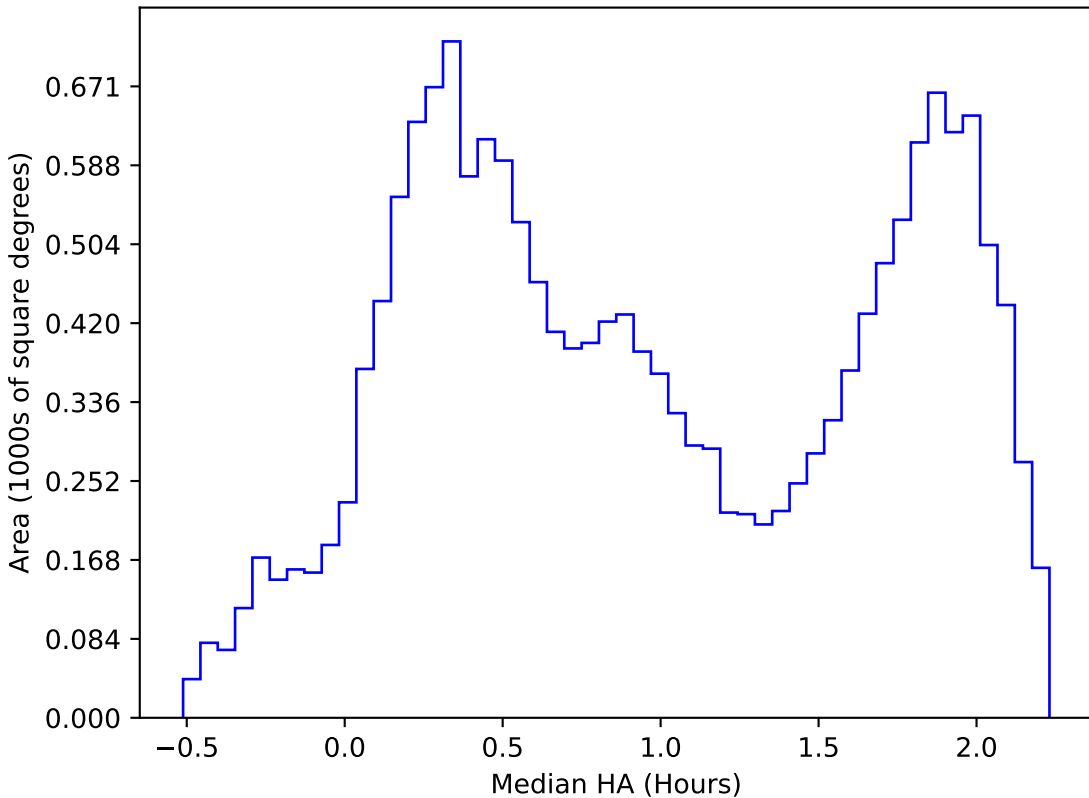
roll_pause_mjdp365_v3.4_10yrs WFD i band: Median HA
