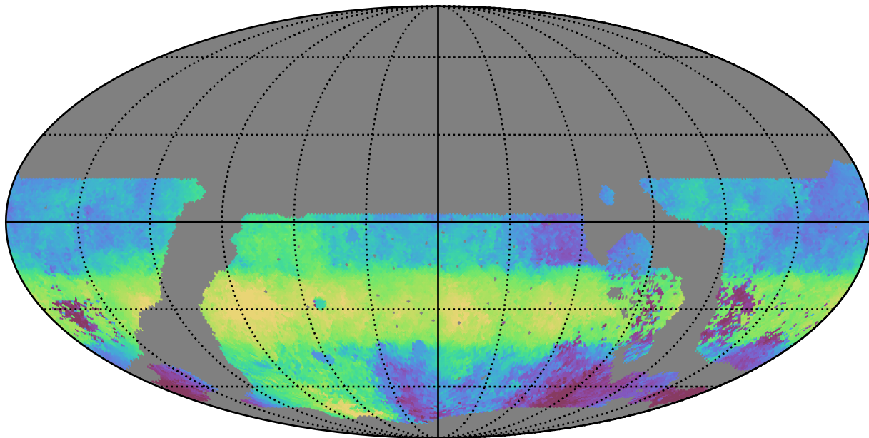
roll_pause_mjdp365_v3.4_10yrs WFD g band: Median HA
