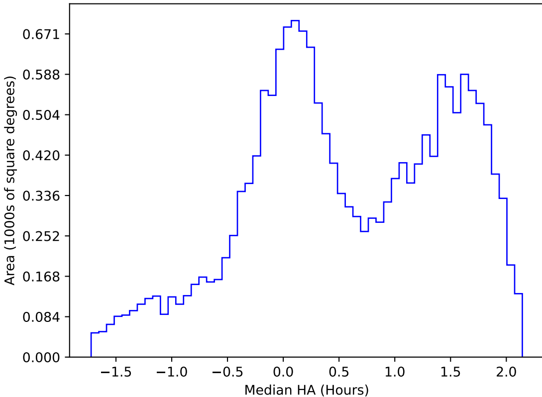
roll_pause_mjdp365_v3.4_10yrs WFD g band: Median HA
