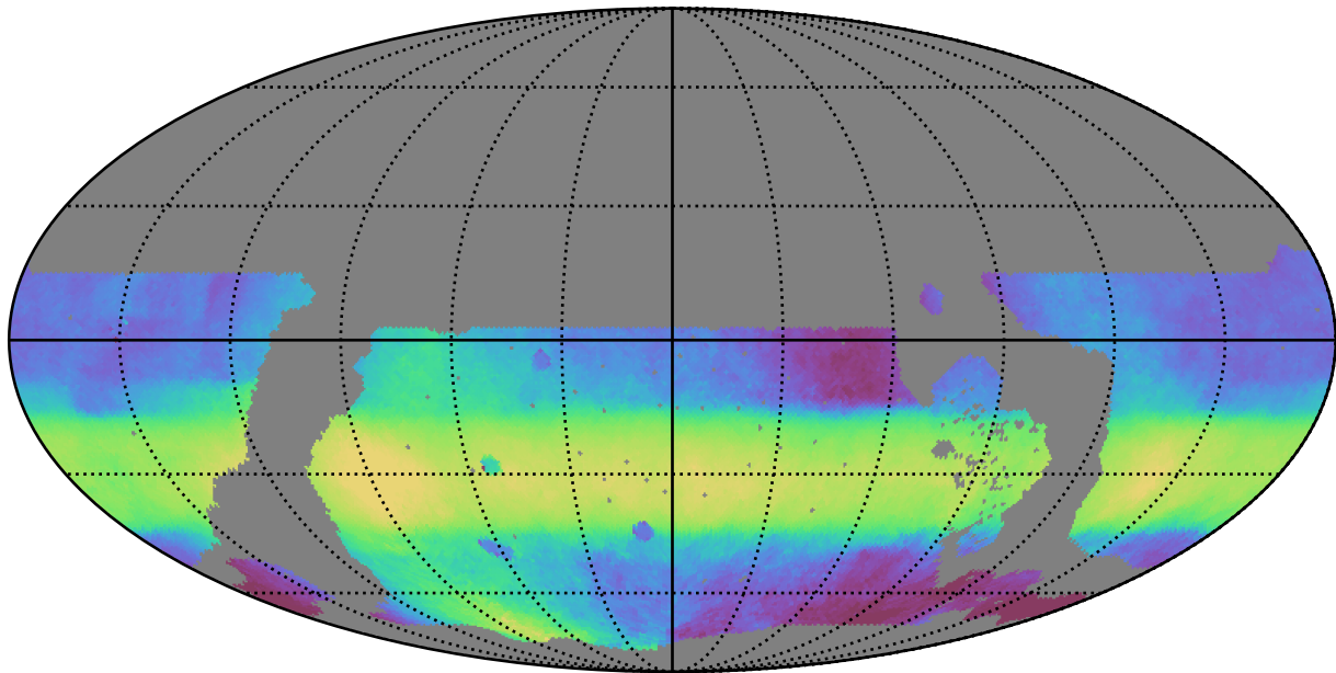
roll_pause_mjdp365_v3.4_10yrs WFD all bands: Median HA
