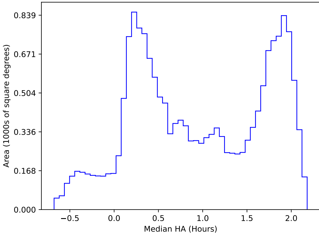
roll_pause_mjdp365_v3.4_10yrs WFD all bands: Median HA
