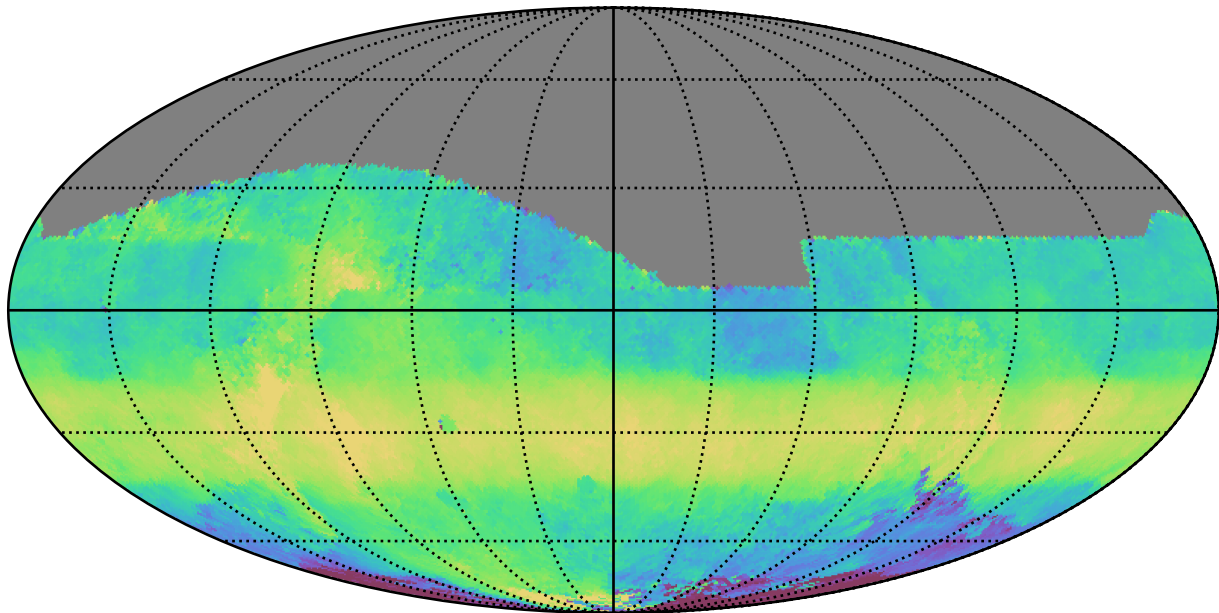
roll_pause_mjdp365_v3.4_10yrs All sky z band: Median HA
