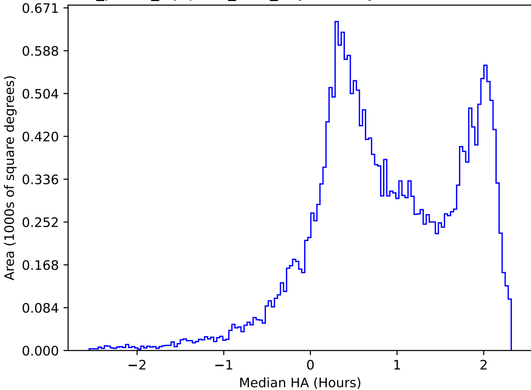
roll_pause_mjdp365_v3.4_10yrs All sky z band: Median HA
