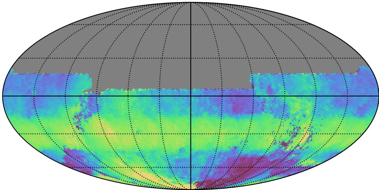
roll_pause_mjdp365_v3.4_10yrs All sky u band: Median HA
