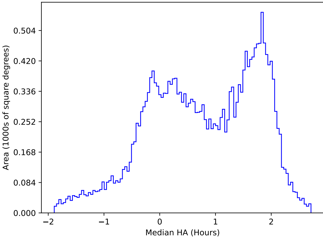
roll_pause_mjdp365_v3.4_10yrs All sky u band: Median HA
