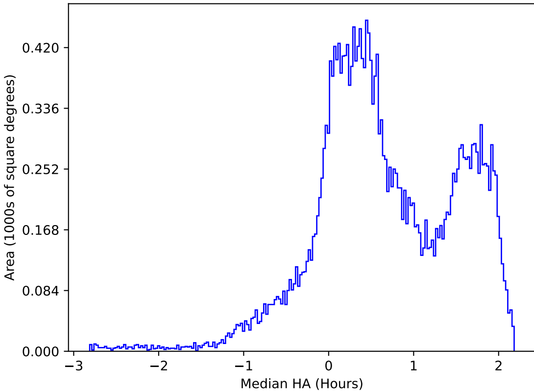
roll_pause_mjdp365_v3.4_10yrs All sky r band: Median HA
