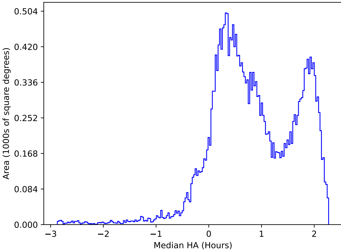
roll_pause_mjdp365_v3.4_10yrs All sky i band: Median HA
