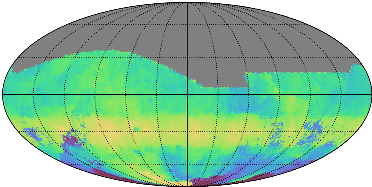
roll_pause_mjdp365_v3.4_10yrs All sky g band: Median HA
