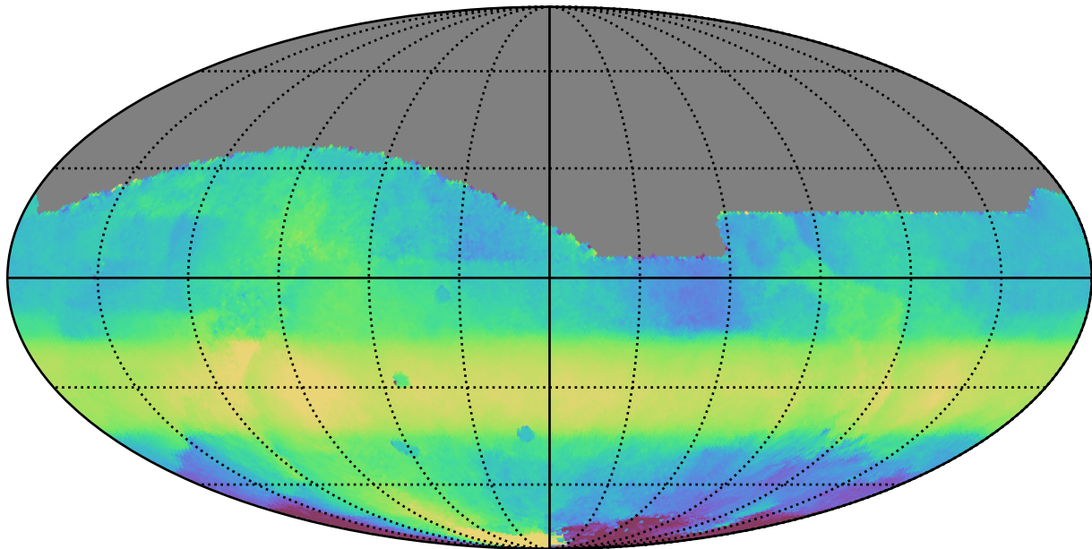
roll_pause_mjdp365_v3.4_10yrs All sky all bands: Median HA
