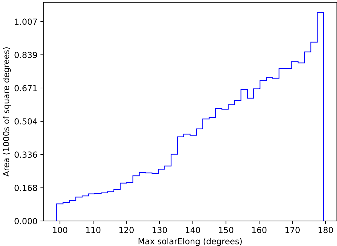
roll_pause_mjdp365_v3.4_10yrs WFD z band: Max solarElong
