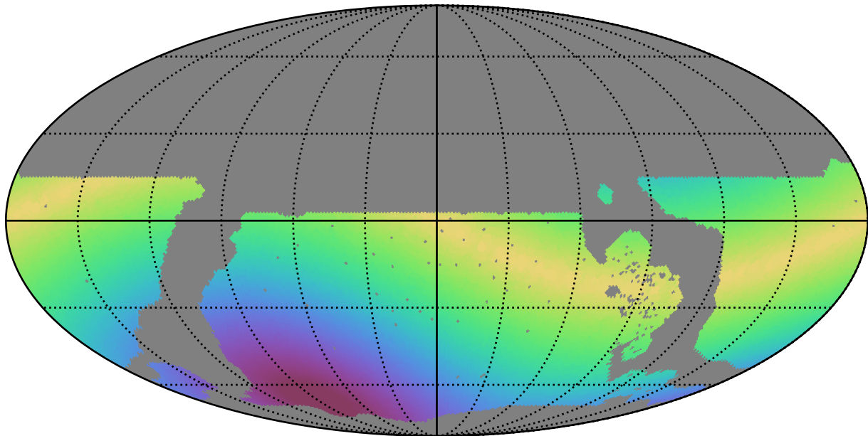
roll_pause_mjdp365_v3.4_10yrs WFD y band: Max solarElong
