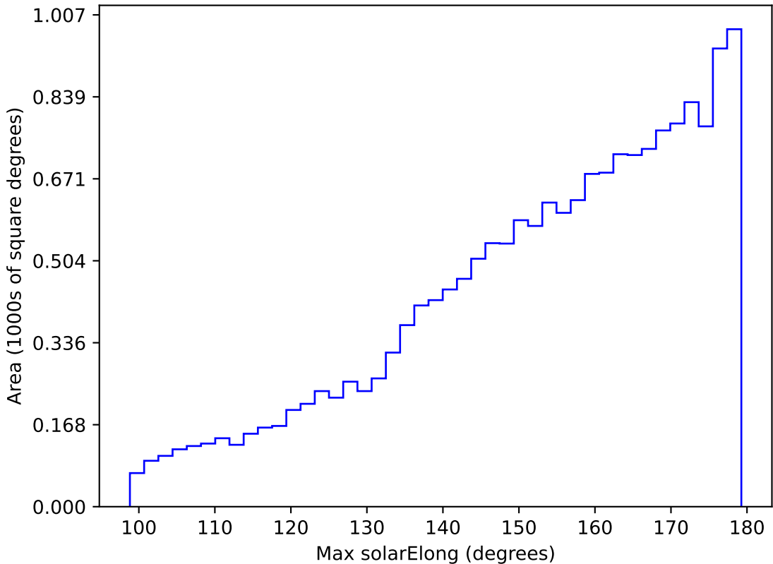
roll_pause_mjdp365_v3.4_10yrs WFD y band: Max solarElong
