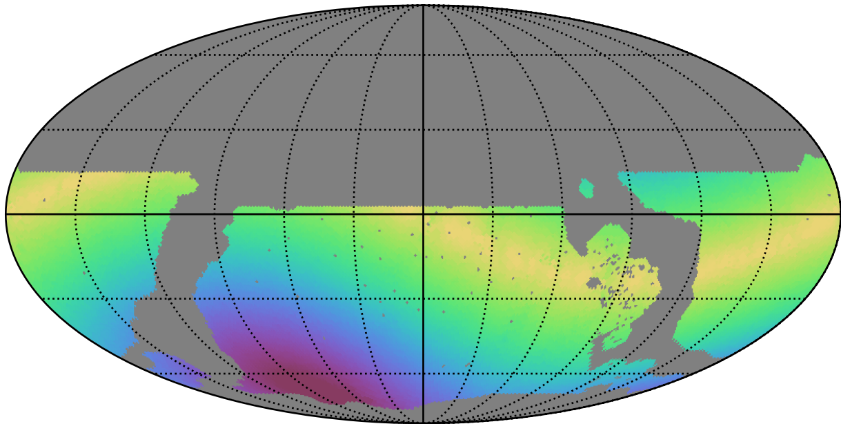
roll_pause_mjdp365_v3.4_10yrs WFD u band: Max solarElong
