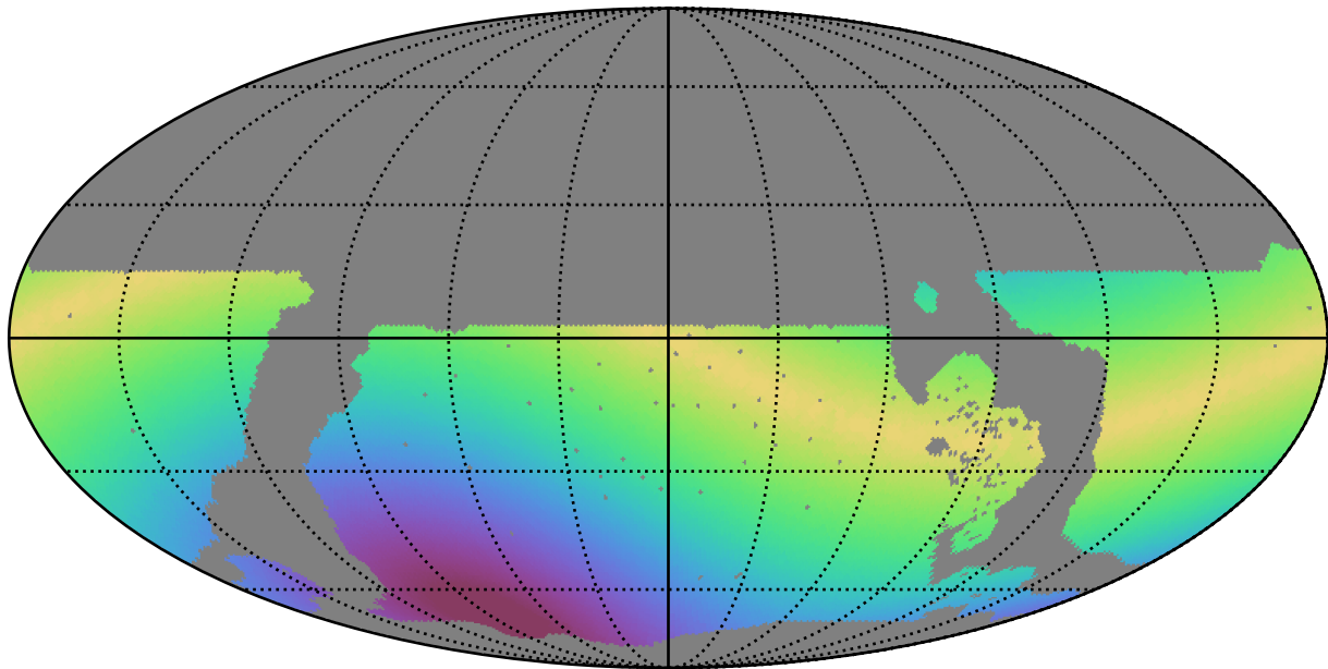
roll_pause_mjdp365_v3.4_10yrs WFD r band: Max solarElong
