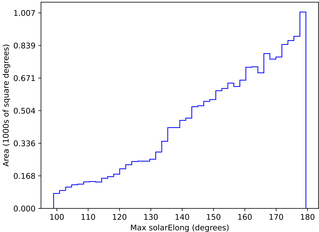
roll_pause_mjdp365_v3.4_10yrs WFD r band: Max solarElong
