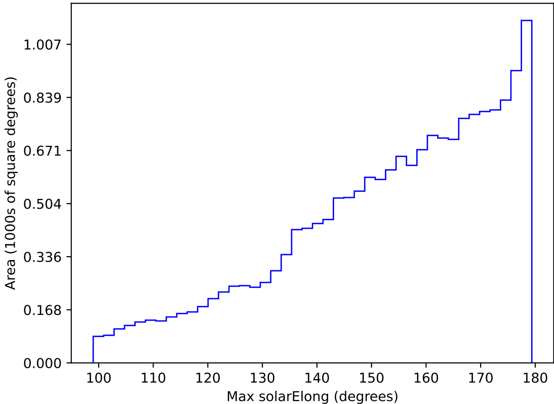
roll_pause_mjdp365_v3.4_10yrs WFD i band: Max solarElong
