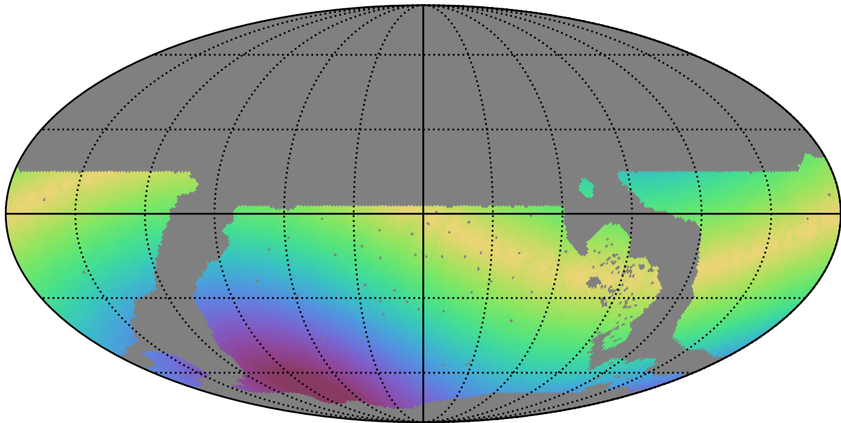
roll_pause_mjdp365_v3.4_10yrs WFD g band: Max solarElong
