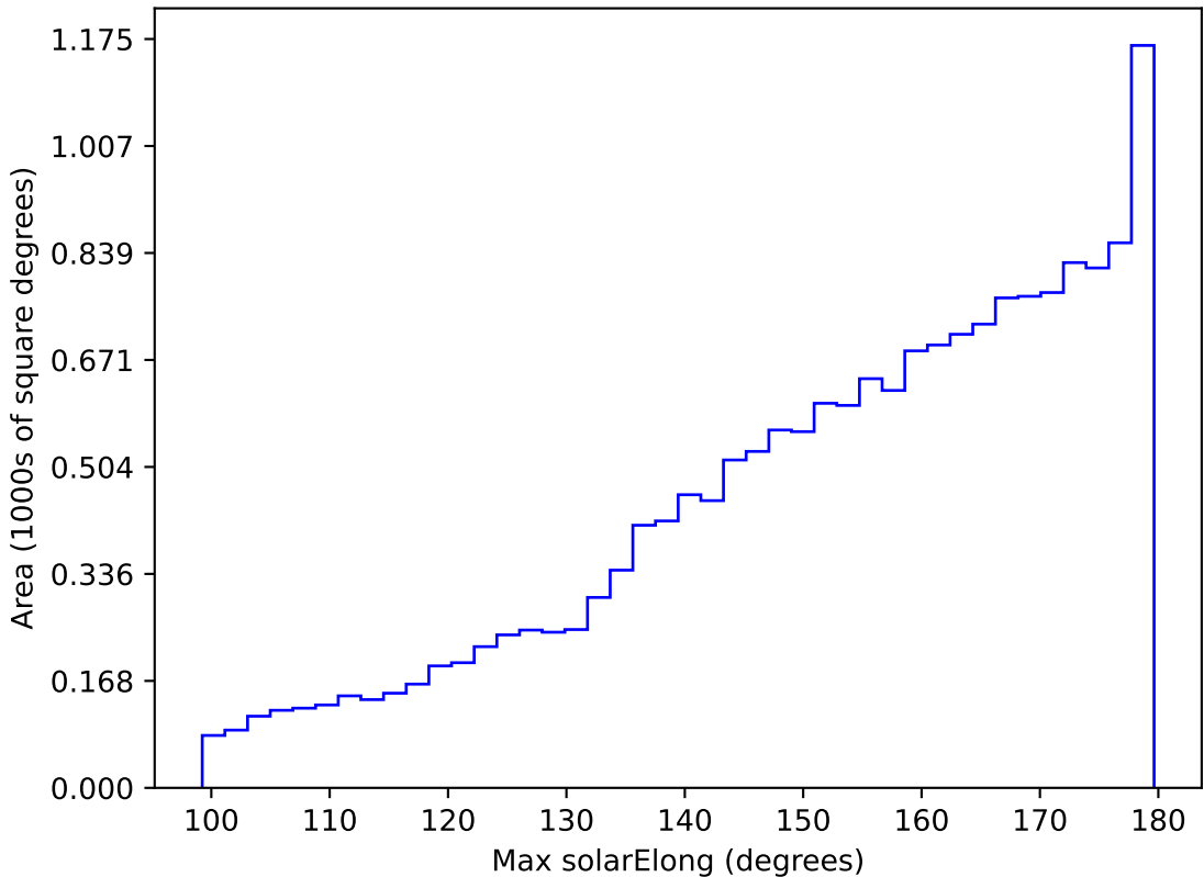
roll_pause_mjdp365_v3.4_10yrs WFD all bands: Max solarElong
