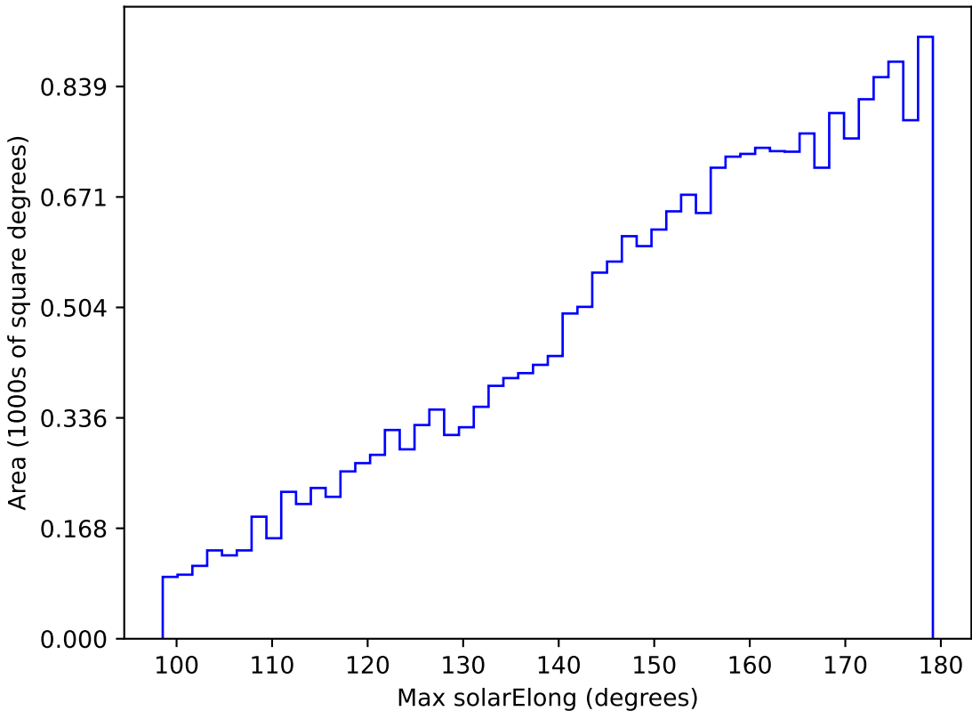
roll_pause_mjdp365_v3.4_10yrs All sky y band: Max solarElong
