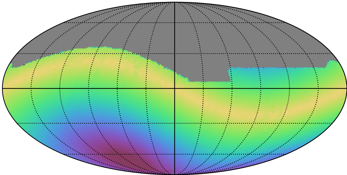
roll_pause_mjdp365_v3.4_10yrs All sky r band: Max solarElong
