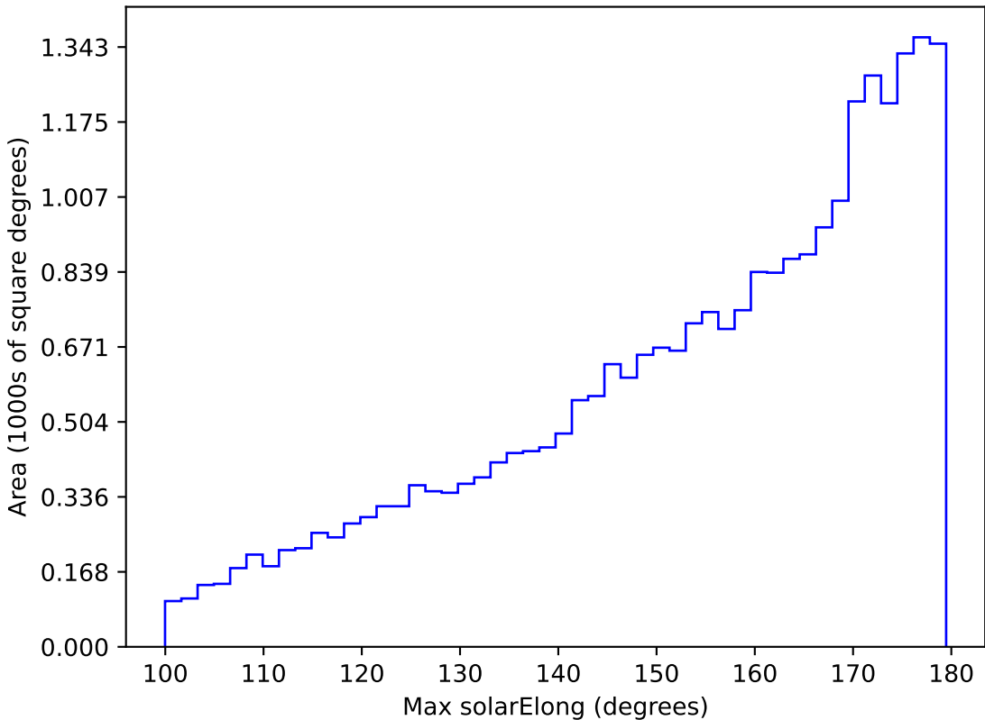
roll_pause_mjdp365_v3.4_10yrs All sky r band: Max solarElong
