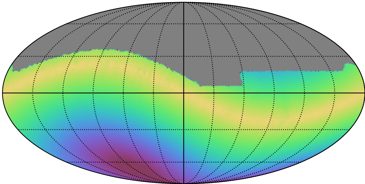
roll_pause_mjdp365_v3.4_10yrs All sky i band: Max solarElong
