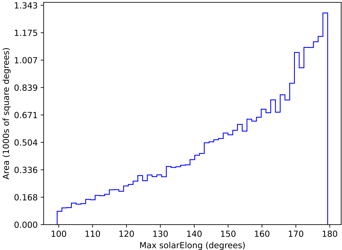
roll_pause_mjdp365_v3.4_10yrs All sky i band: Max solarElong
