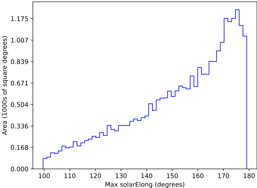
roll_pause_mjdp365_v3.4_10yrs All sky g band: Max solarElong
