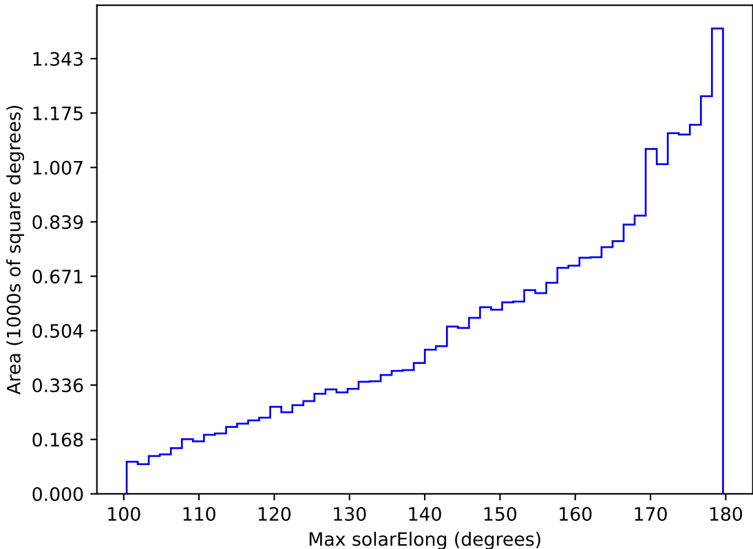
roll_pause_mjdp365_v3.4_10yrs All sky all bands: Max solarElong
