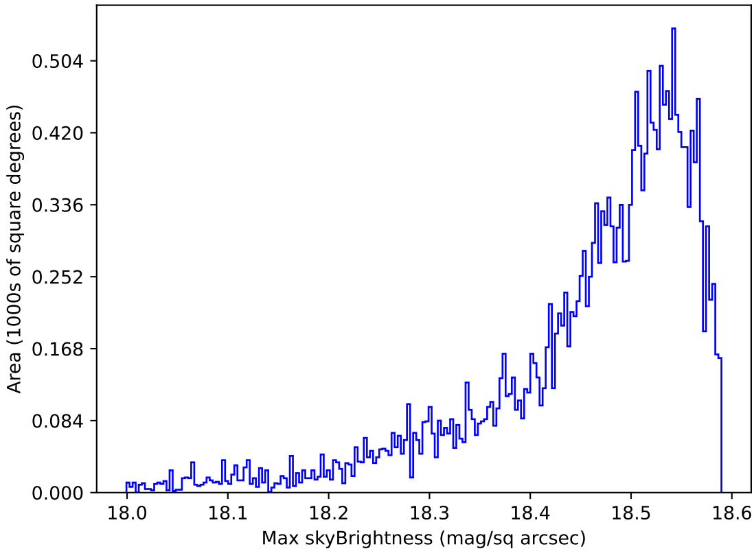
roll_pause_mjdp365_v3.4_10yrs Yr 1 y band: Max skyBrightness
