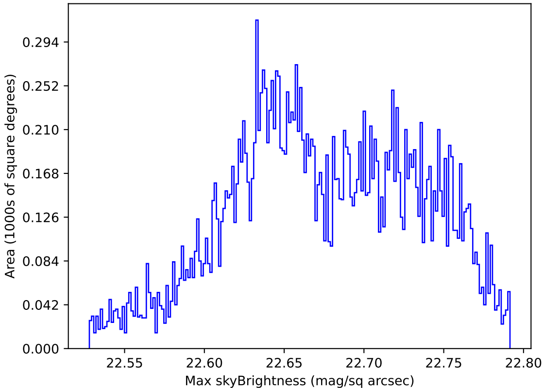
roll_pause_mjdp365_v3.4_10yrs Yr 1 u band: Max skyBrightness
