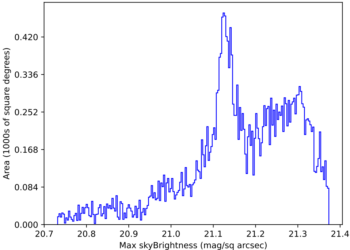
roll_pause_mjdp365_v3.4_10yrs Yr 1 r band: Max skyBrightness
