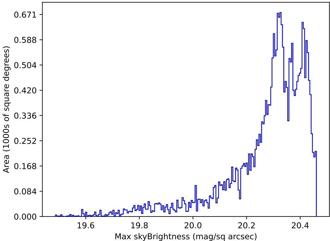
roll_pause_mjdp365_v3.4_10yrs Yr 1 i band: Max skyBrightness
