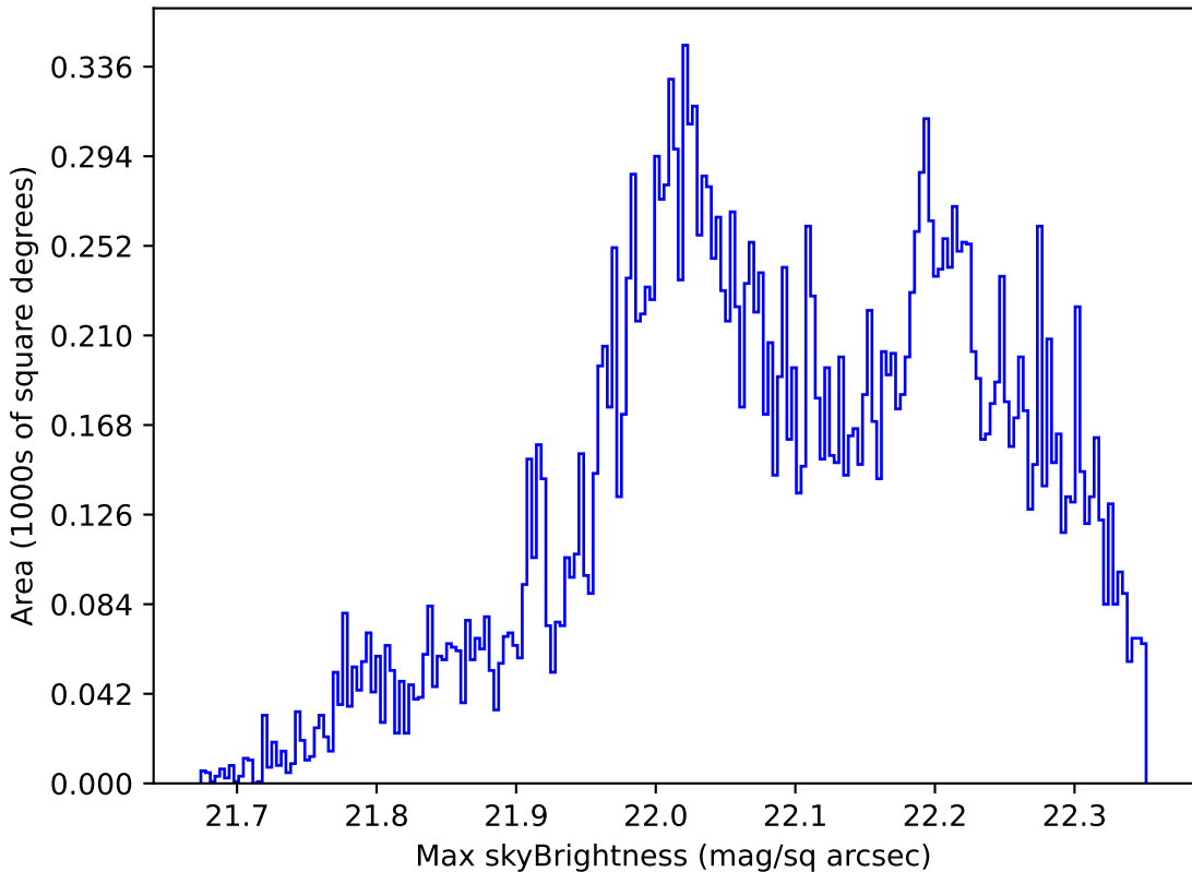
roll_pause_mjdp365_v3.4_10yrs Yr 1 g band: Max skyBrightness
