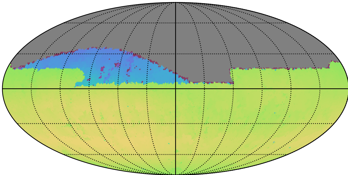
roll_pause_mjdp365_v3.4_10yrs Yr 1 all bands: Max skyBrightness
