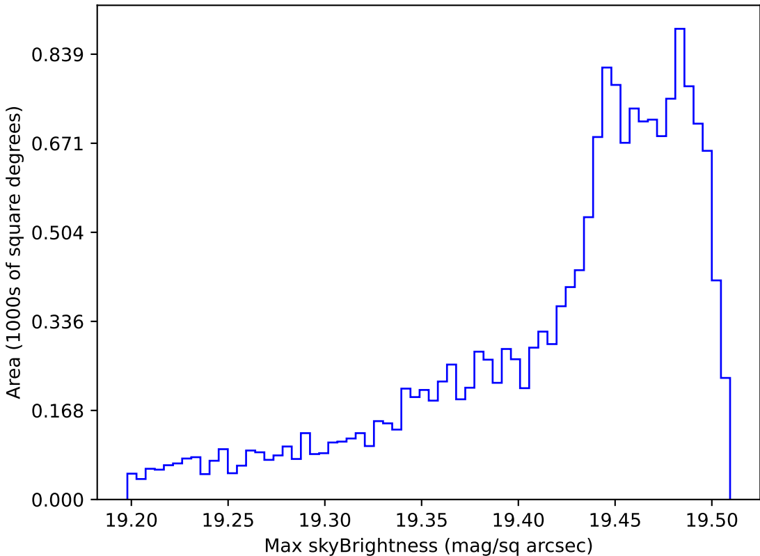
roll_pause_mjdp365_v3.4_10yrs WFD z band: Max skyBrightness
