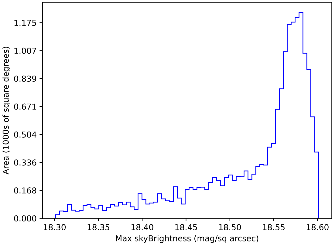
roll_pause_mjdp365_v3.4_10yrs WFD y band: Max skyBrightness
