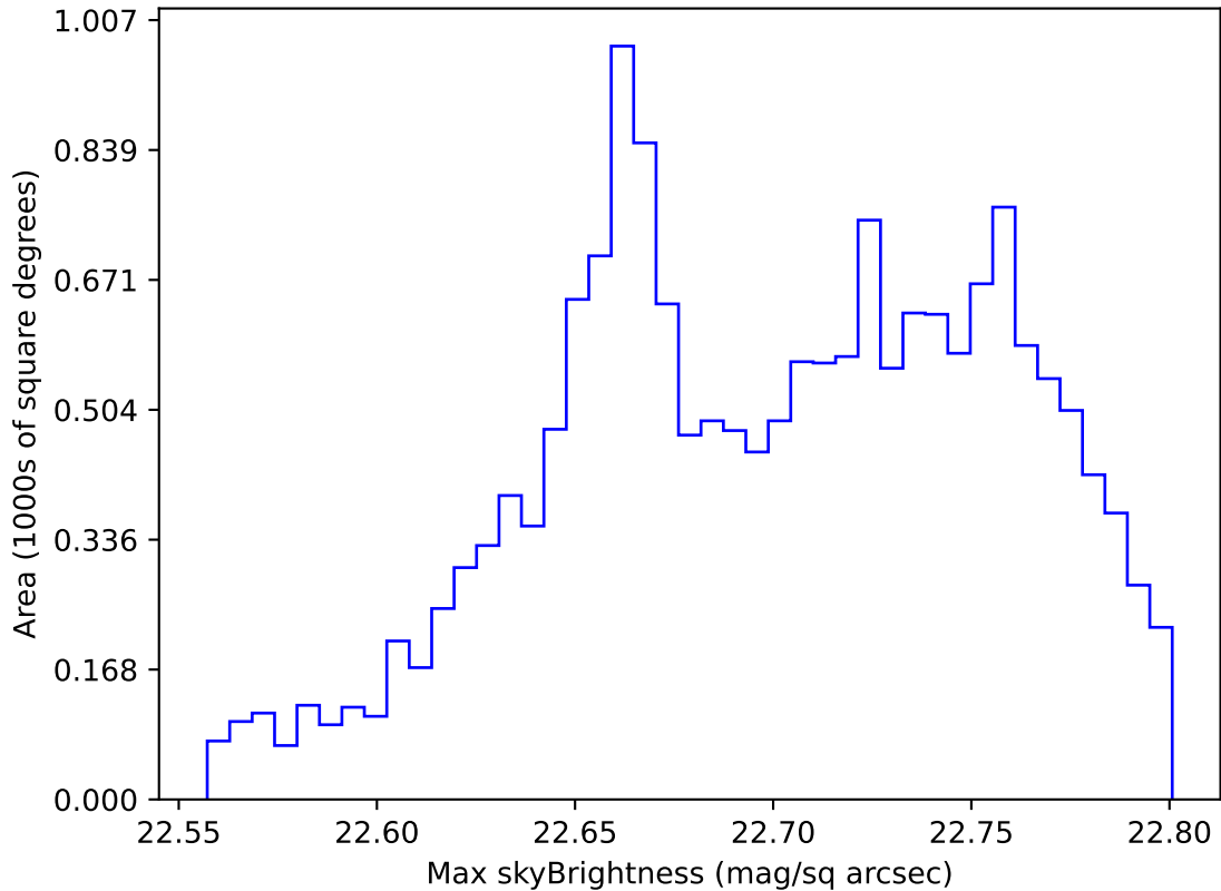
roll_pause_mjdp365_v3.4_10yrs WFD u band: Max skyBrightness
