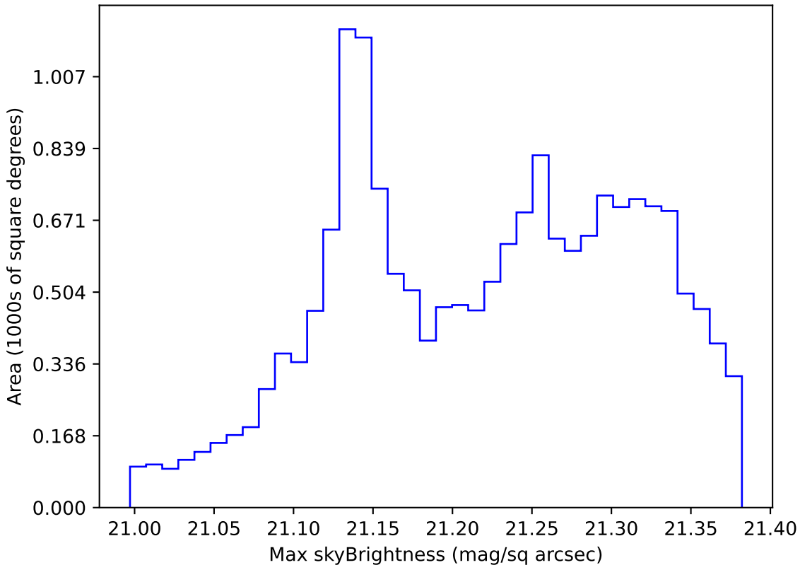
roll_pause_mjdp365_v3.4_10yrs WFD r band: Max skyBrightness
