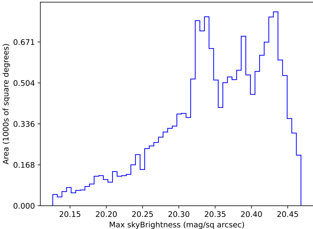
roll_pause_mjdp365_v3.4_10yrs WFD i band: Max skyBrightness
