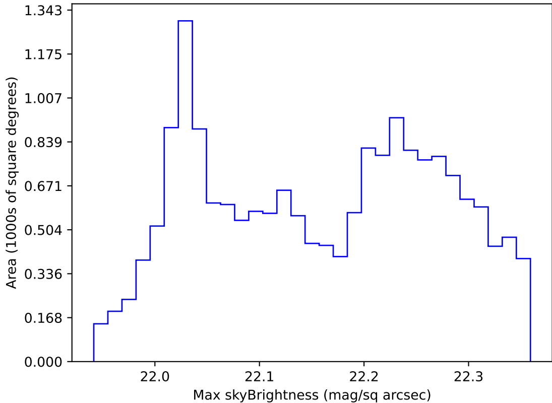
roll_pause_mjdp365_v3.4_10yrs WFD g band: Max skyBrightness
