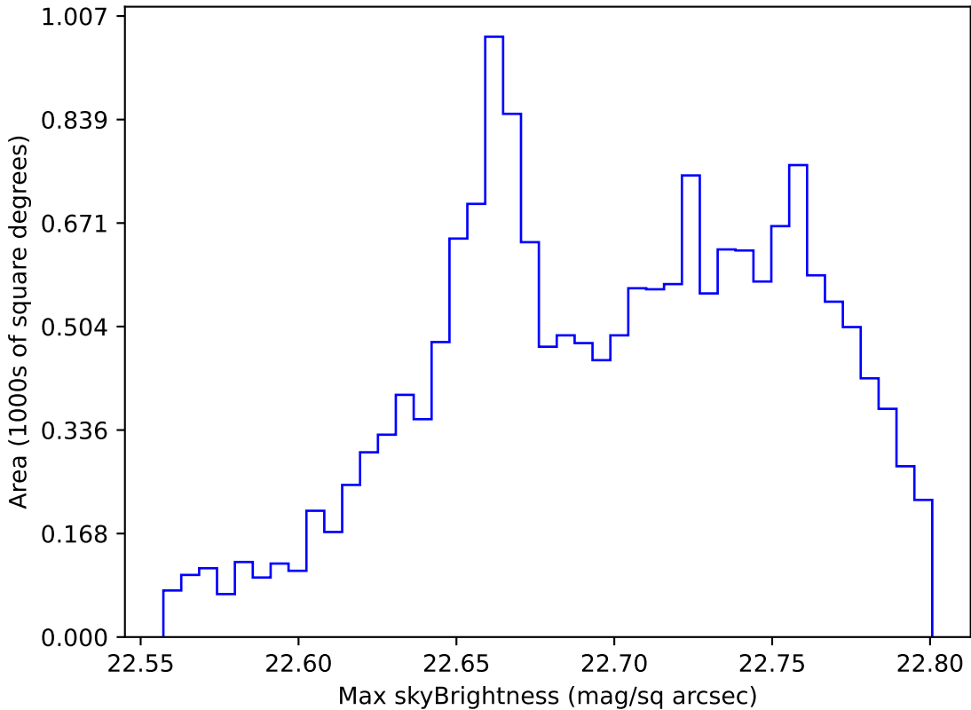
roll_pause_mjdp365_v3.4_10yrs WFD all bands: Max skyBrightness
