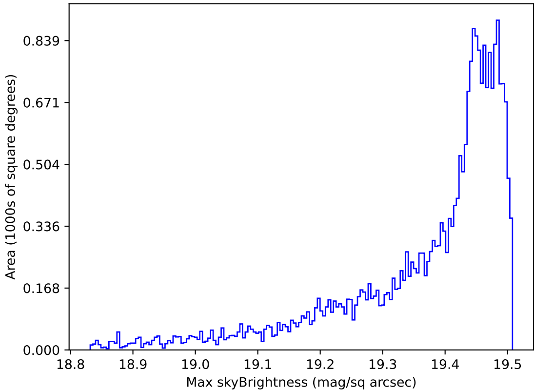
roll_pause_mjdp365_v3.4_10yrs All sky z band: Max skyBrightness
